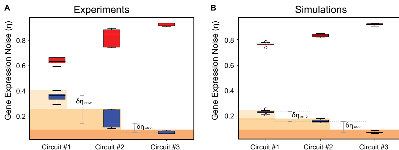
Figure 5. Apparent extrinsic and intrinsic noise. Extrinsic (red) and intrinsic (blue) noise values of three circuit designs. The box height indicates the 75% (top) and 25% (bottom) quantiles and the whiskers bound the upper and lower range of values observed. (A) Noise decomposition of the experimental data for the three circuit designs. (B) Noise decomposition of the simulated data for the three circuit designs. In both cases, the extrinsic noise appears to increase while the intrinsic noise appears to decrease as the two proteins become coupled (at transcription, translation, post-translation levels)
