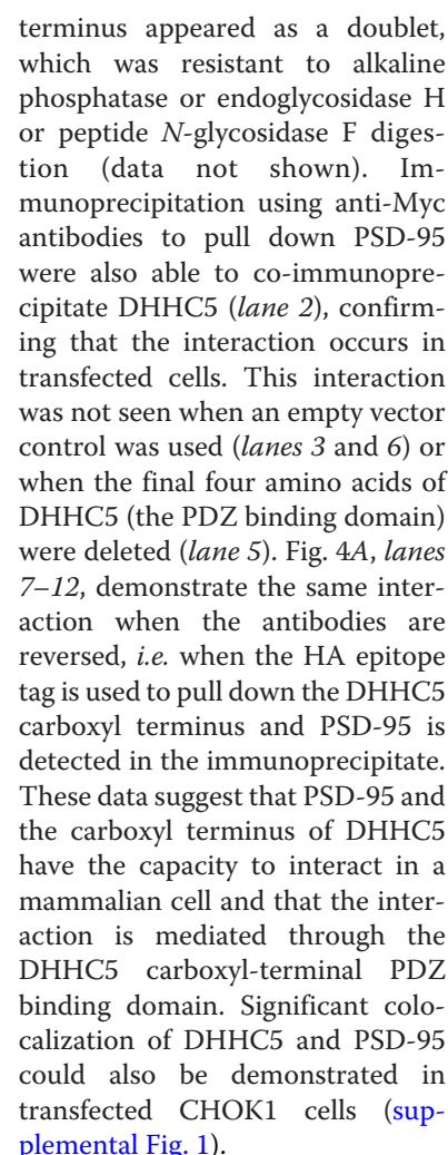
To determine whether an endogenous interaction between DHHC5 and PSD-95 could be detected, mouse brain membranes were extracted using a stringent protocol that employs membrane solubilization in 1% sodium deoxycholate. As shown in Fig. 4B, when PSD-95 was immunoprecipitated from brain lysates, DHHC5 was also found in the immunoprecipitates (Fig. 4B, lanes 1–3). The DHHC5 signal was absent from similarly prepared brain lysates obtained from gene-targeted DHHC5 mice (Fig. 4B, lanes 4–6). We were
